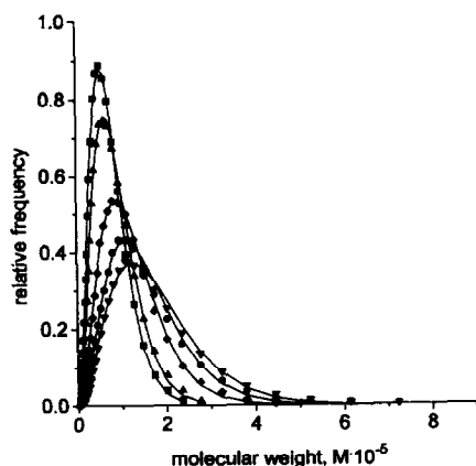
Fig. 7. Molecular weight distributions of poly(styrene-co-acrylonitrile)s after normalization no. 2; relative concentration vs molecular weight. Symbols represent experimental data, solid lines indicate Schulz distribution function fits. Significant change in molecular weight distribution width is not reflected in the polydispersity index change ( I = 1.6 – 1.7 for all curves).
